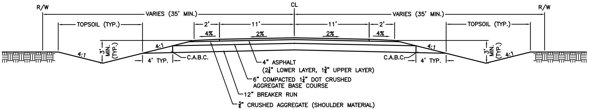
TYPICAL MINIMUM RURAL STREET SECTION
