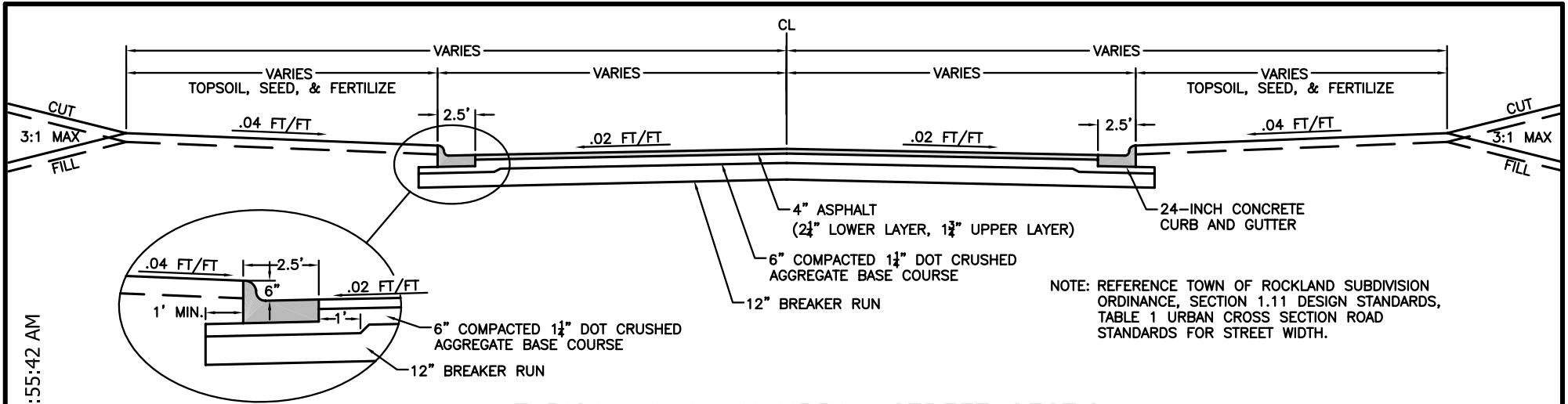
TYPICAL MINIMUM URBAN STREET SECTION
